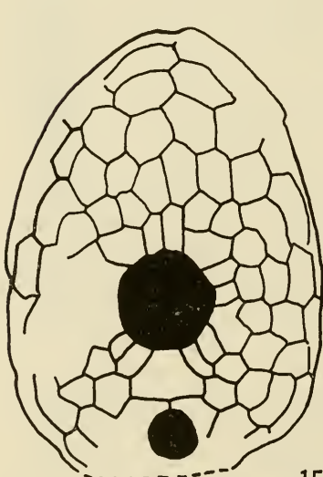
FIGURES 13-16.— Echinocyamus bisexus Kier, new species. 13, Adapical view of USNM 650745 from the test well level 1130-1135 feet showing the large and widely separated genital pores, which suggest that this individual was a female; \times 12. 14, Adapical view of the holotype, USNM 650722, showing the smaller, closely situated genital pores, which suggest that this specimen was a male as opposed to the female in Figure 13; test well level 1130-1135 feet; \times 14. 15, Adoral view of USNM 650748 showing the plate arrangement in a small specimen as contrasted to the larger specimen in Figure 16 (USNM 650746—1135-1160 feet). Note that the first coronal plates are smaller and the peristome larger than in the larger specimen.
