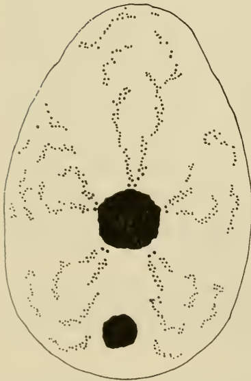
FIGURES 19-22.— Echinocyamus bisexus Kier, new species. 19, Adoral view of smallest specimen in the collection showing the widely separated genital pores. Presumably when the genital pores are first introduced in the female, they are this far apart. Note the periproct partially visible from above; USNM 650721 from the test well level 1130-1135 feet; \times 40 . 20, Adoral view of same specimen showing the large peristome; \times 40 . 21, Adoral view of a female specimen, USNM 650723, from the test well level 1135-1145 feet showing the arrangement of the accessory pores; \times 14 . 22, View of interior of USNM 650747 showing the position of the interior supports; test well level 1130-1135 feet; \times 20 .
