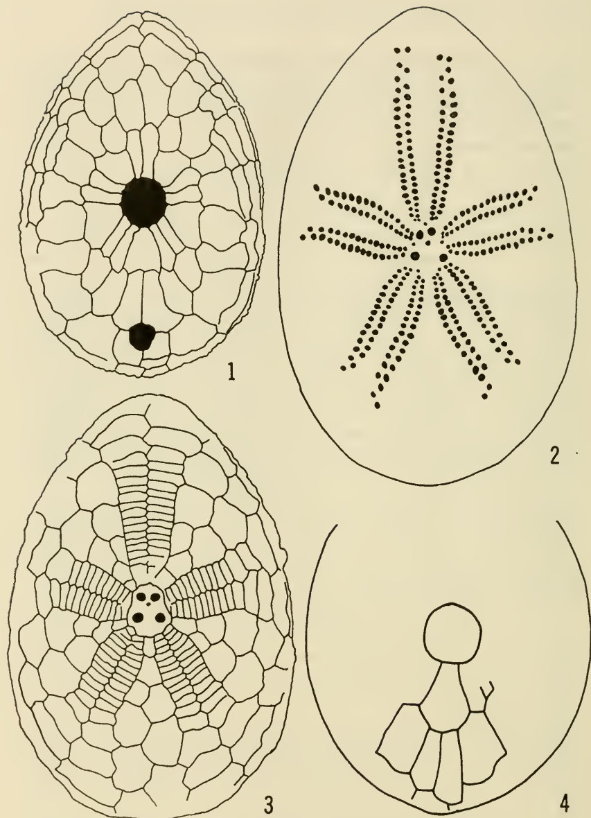
FIGURES 1-4.—1-3, Leniechinus herricki Kier, new species. 1, Adoral view of USNM 650749 from the test well level 1135-1160 feet showing the plate arrangement; \times 10 . 2, Adapical view of the holotype, USNM 650717, from the test well 1135 feet; \times 10 . 3, Adapical view of USNM 650750 showing the plate arrangement; \times 10 . 4, Lenita patellaris (Leske). Adoral view showing plate arrangement, where visible, of a specimen from the middle Eocene, Parney, France, from the Michelin collection, Laboratoire de Paléontologie, Institut de Géologie, Université de Paris, Orsay; \times 15 .
