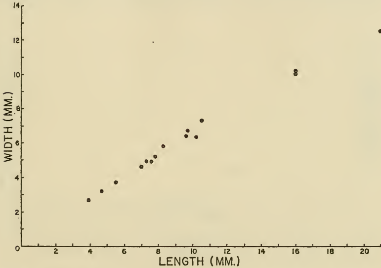
FIGURE 5.— Lenechinus herricki Kier, new species. Scattergram of the length and width showing the slight variation in the length-width ratio.
