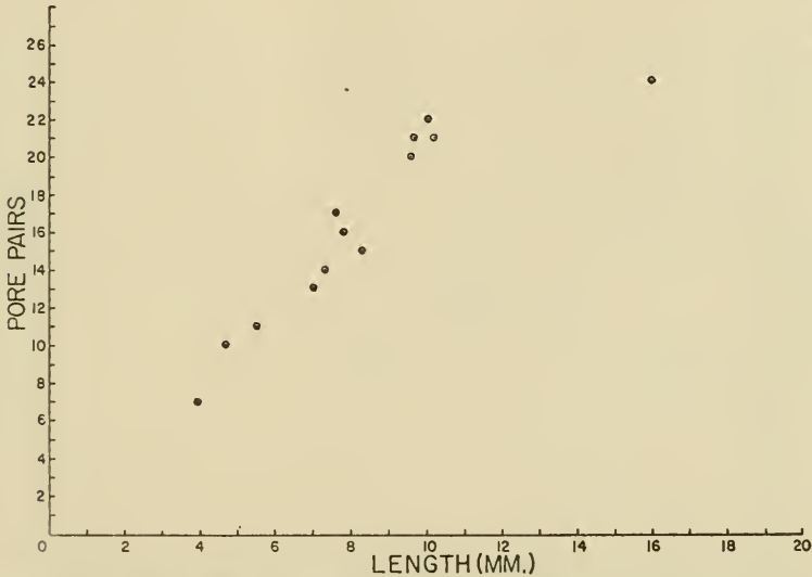
FIGURE 9.— Lenechinus herricki Kier, new species. Scattergram showing the number of pore-pairs in a single poriferous zone of petal III. As evident from the curve in the path of the points, new pore-pairs are introduced at a slower rate after the echinoid exceeds 10 mm in length.
