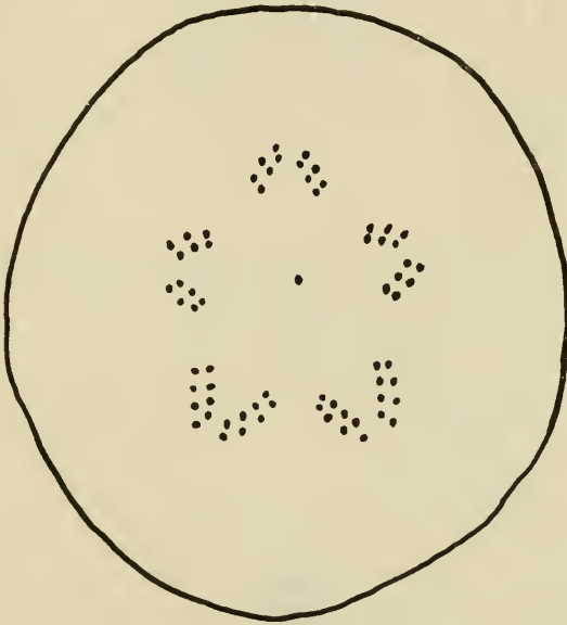
FIGURE 37.— Durhamella cf. D. floridana (Twitchell). Adapical view of a small specimen showing the lack of genital pores and the few petaloid pore-pairs; test well level 1135-1145 feet; \times 24 .
