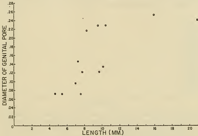
FIGURE 7.— Leniechinus herricki Kier, new species. Scattergram showing the great variation in the diameter of the genital pores. The lack of separation of the points into two distinct paths suggests sexual dimorphism.
