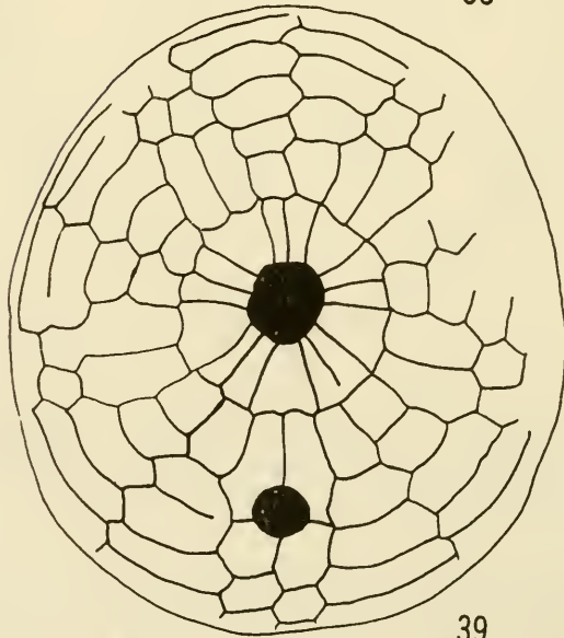
FIGURES 38-39.— Durhamella cf. D. floridana (Twitchell). 38, Adapical view showing the petaloid pores in USNM 650738 from the test well level 1135-1160 feet. A photograph of this specimen is on plate 10, figure 1; \times 5 . 39, Adoral view of USNM 650751 from the test well level 1135 feet showing the plate arrangement in a small specimen as compared to a large specimen illustrated in Figure 40. Note the smaller first coronal plates in the smaller specimen; \times 15 .
